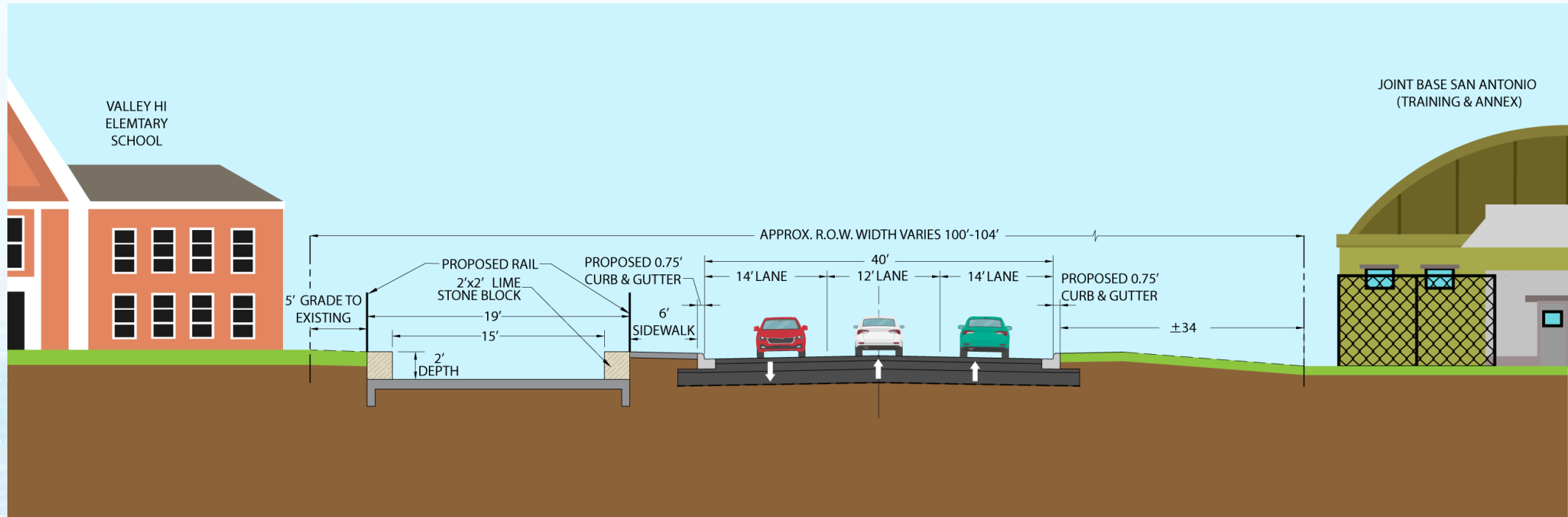
PROPOSED RAY ELLISON BLVD TYPICAL SECTION (STA 21+00 TO 25+00)
