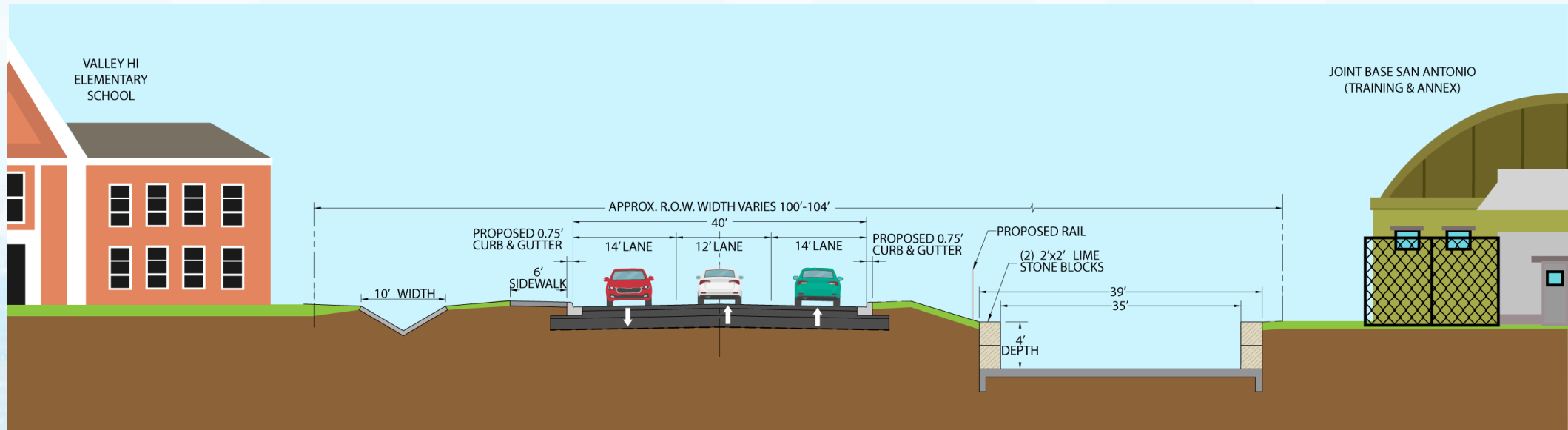
PROPOSED RAY ELLISON BLVD TYPICAL SECTION (STA 17+00 TO 21+00)
