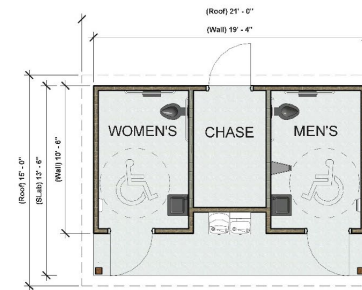
① FLOOR PLAN
